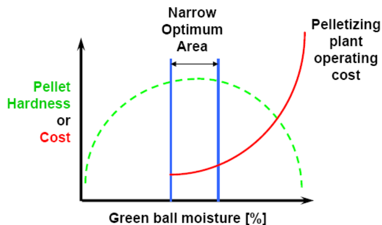
Figure 1: Optimal green ball moisture vs. operational cost and pellet hardness
