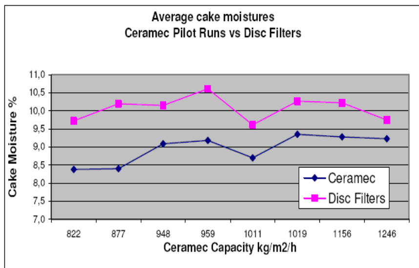
Fig. 9: Cake moisture - RVDF vs. Ceramec®
