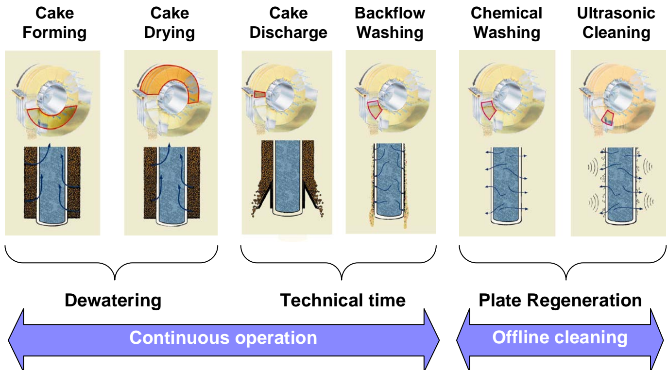
Fig. 4: Operational principle of Ceramec ® filter
