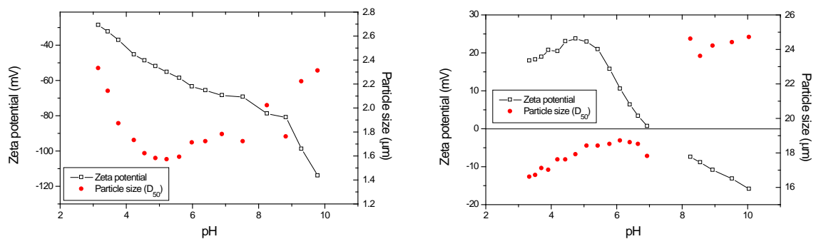
Fig.2a/b: Zeta potential vs. Silica particle size (left) vs. Iron oxide particle size (right) 3)
