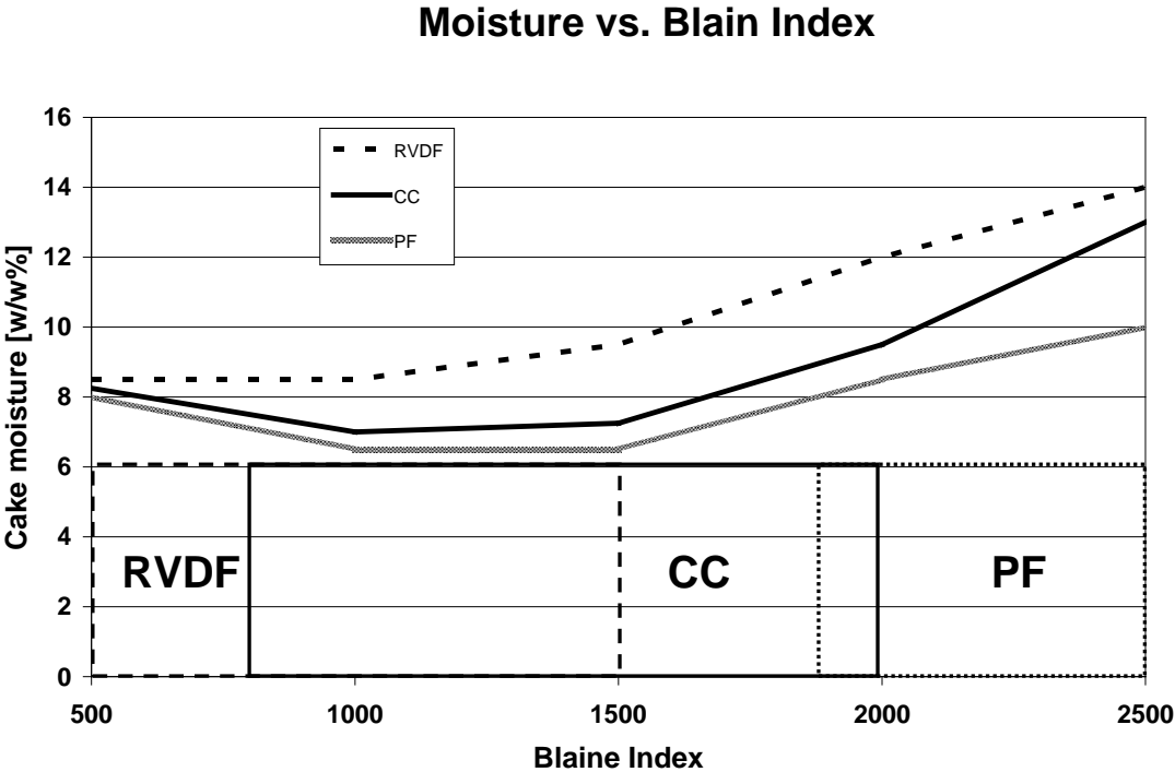
Fig. 10: Rough selection of filtration equipment
